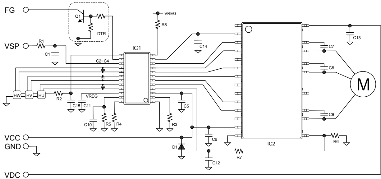
Figure 33. Application circuit example (150° commutation driver)
