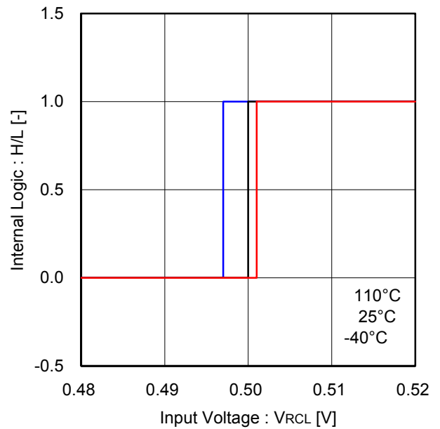
Figure 24. RCL input threshold voltage
