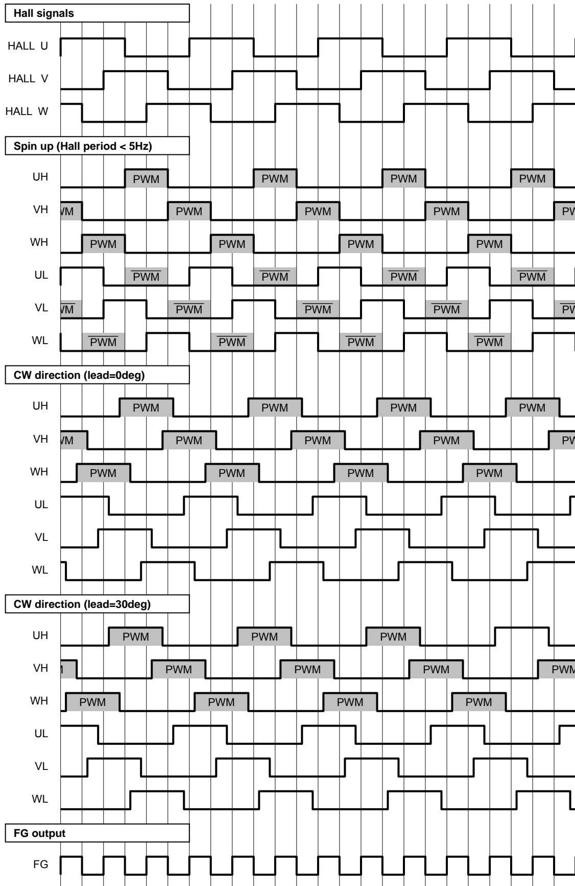
Figure 7. BD62013AFS (Clockwise) timing charts
