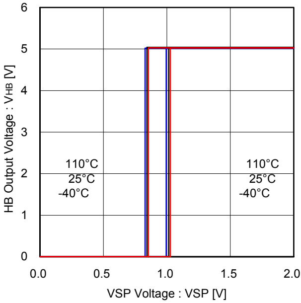
Figure 25. HB enable voltage
