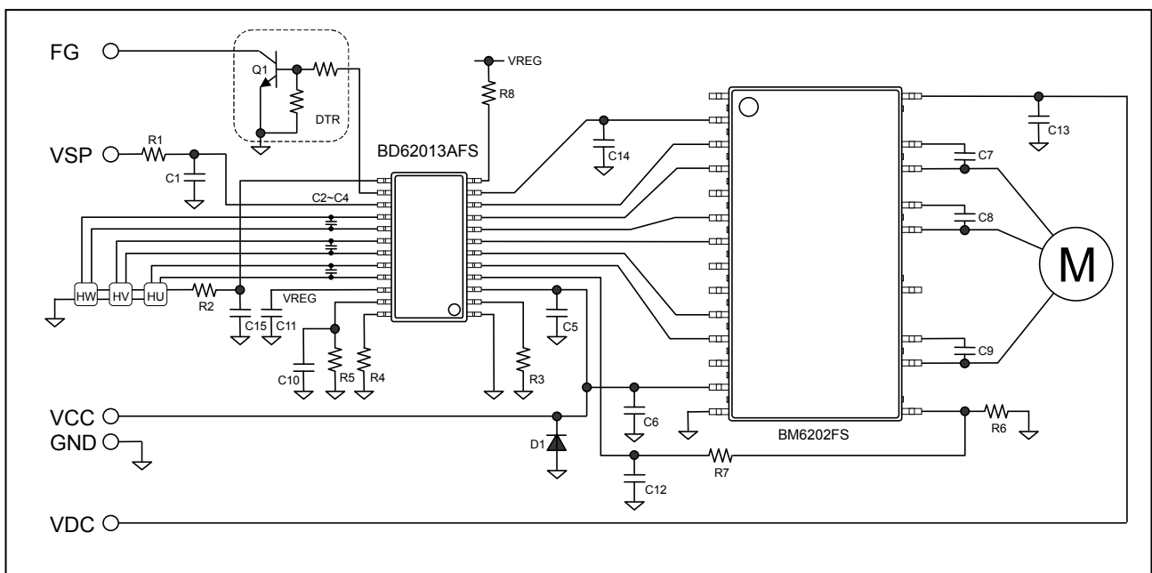
Figure 1. Application circuit example - BD62013AFS & BM6202FS
