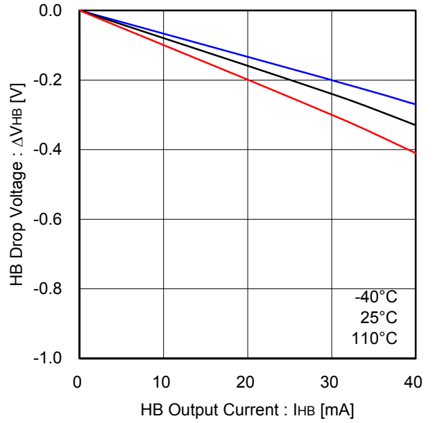
Figure 26. HB output drive capability
